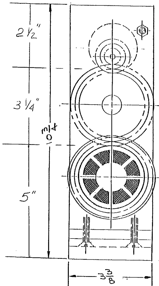
MINI BARREL ASSEMBLY 2 1/2" X 2 3/4" Long AND 2 1/2" X 4" Long
